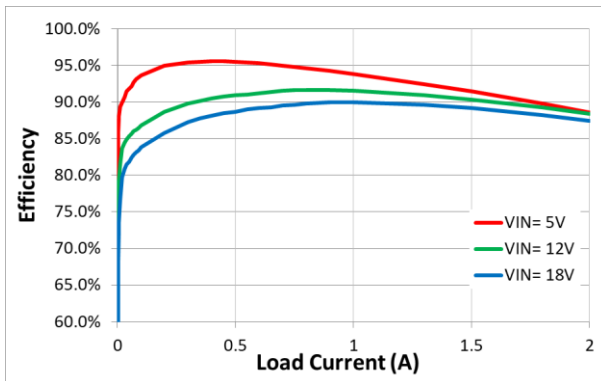
Figure 1. Efficiency vs. Load Current ( V_{OUT}=3.3V , L=3.3\mu H )
