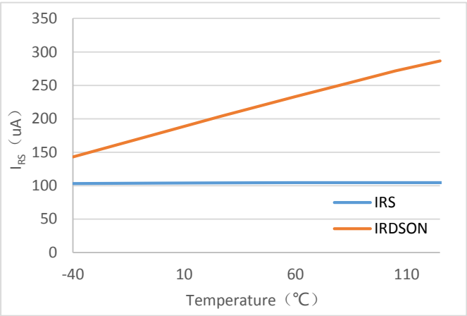
Figure 5. ILIM Current Source vs Junction Temperature
