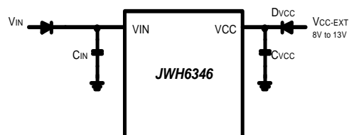
Figure13. VCC Bias Supply Connection From V OUT or Auxiliary Supply
