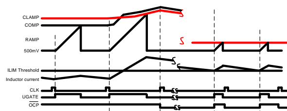
Figure16. OCP Duty Cycle Limiting Waveforms
