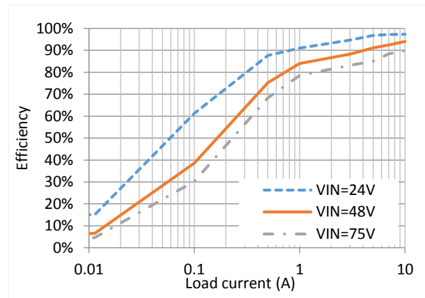
Figure 7. Efficiency vs Load Current
