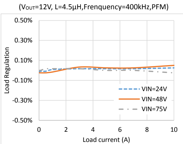
Figure 8. Load Regulation
