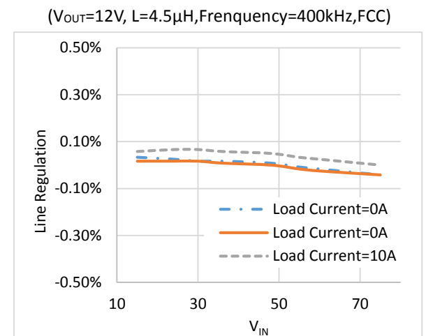
Figure 9. Line Regulation
