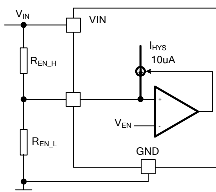
Figure12. UVLO Setting
