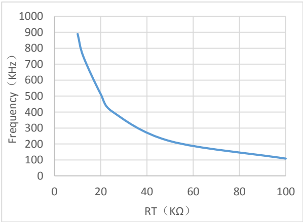
Figure 4. Switch Frequency vs RT
