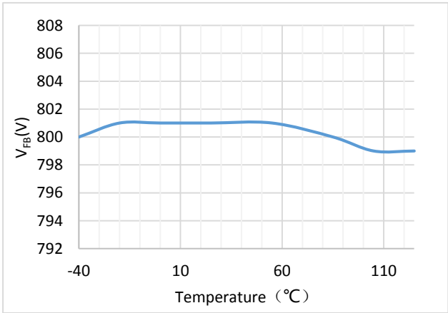
Figure 3. FB Voltage Regulation vs Junction Temperature
