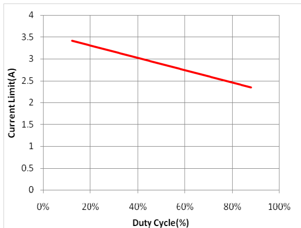
Figure 3. Duty Cycle vs Current Limit
