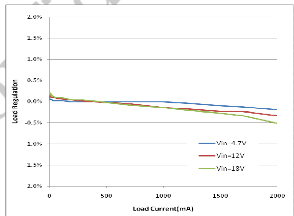
Figure 4. Output Voltage Regulation vs Load Current ( V_{out}=3.3V , L=3.3\mu H )
