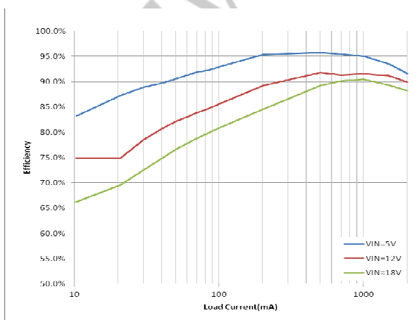
Figure 5. Efficiency vs Load Current (V out =3.3V, TSOT23-6)
