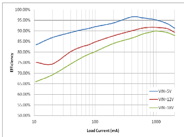
Figure 6. Efficiency vs Load Current (V out =3.3V, SOT563)
